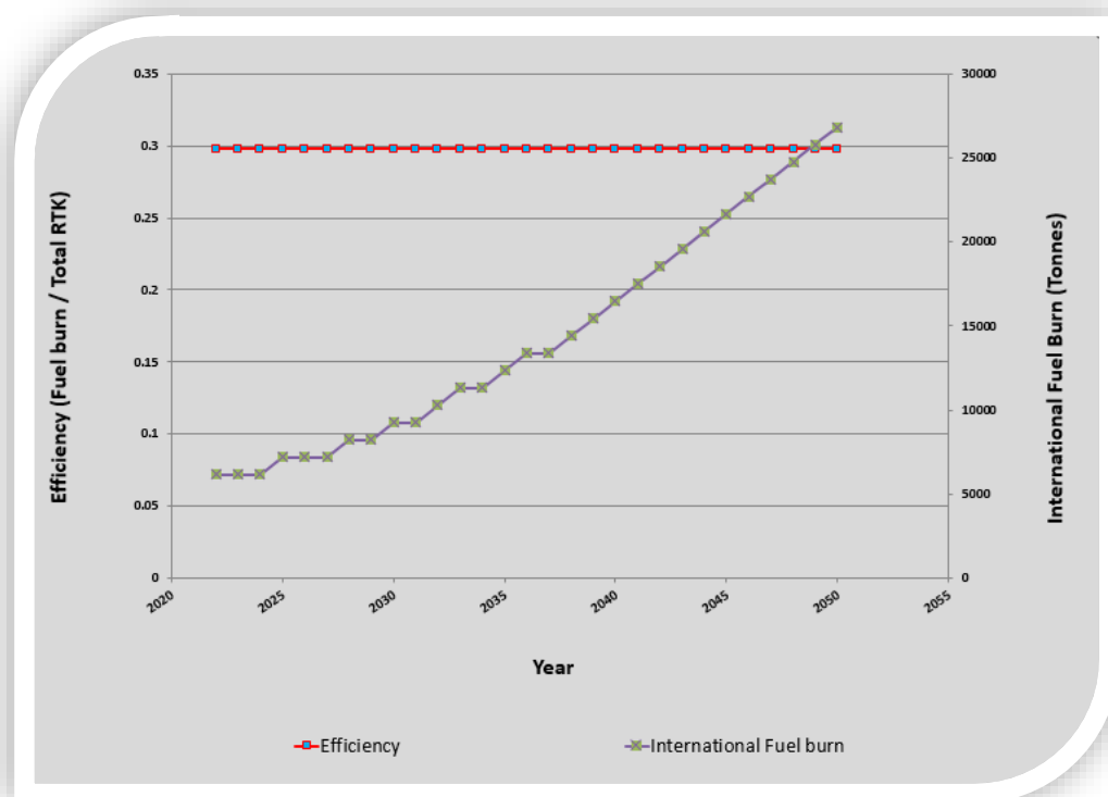
Figure 2. Graph of Baseline Scenario for International Flight
