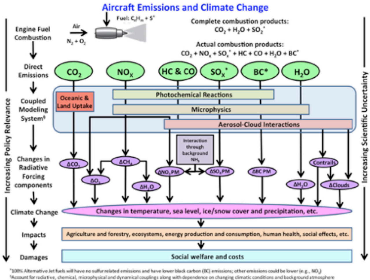
Figure 1. Updated schematic of the principal emissions from aviation operations and the relationship of emissions to climate change and impacts. The terminology, \Delta X , indicates a change in component X. The term, \Delta clouds , represents contrail-induced cloudiness and aerosol-cloud interactions. (From Brasseur et al. , 2015).
